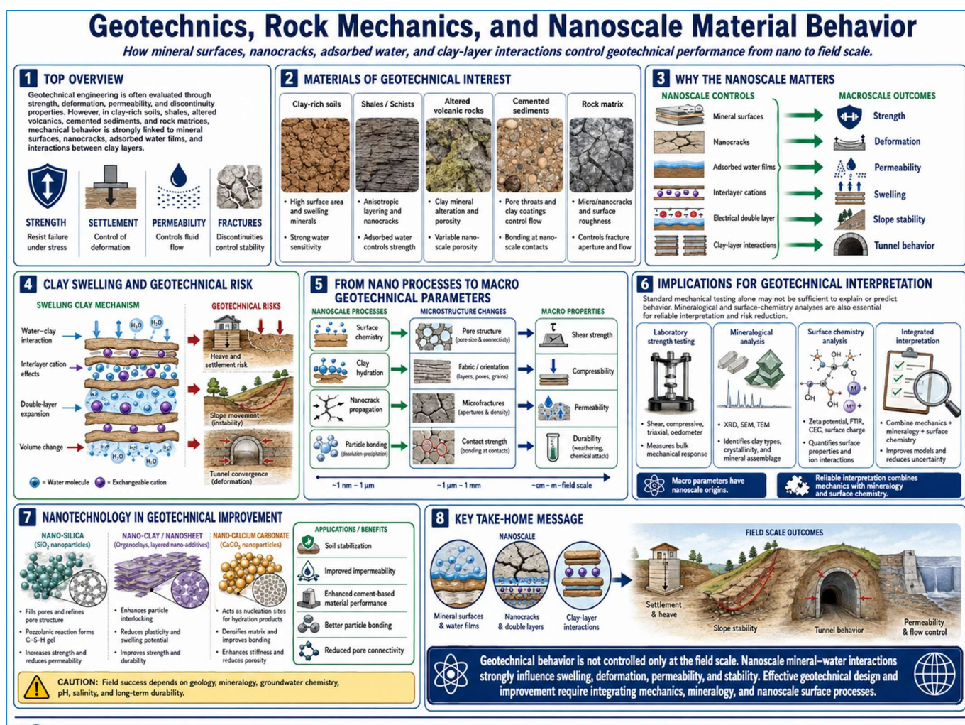
Fig. 9. Geotechnical and rock-mechanics implications of nanoscale fabric, clay-water interactions, nano-cracks, and engineered nanomaterials (compiled from Bergaya and Lagaly, 2013; Diab et al., 2026)
