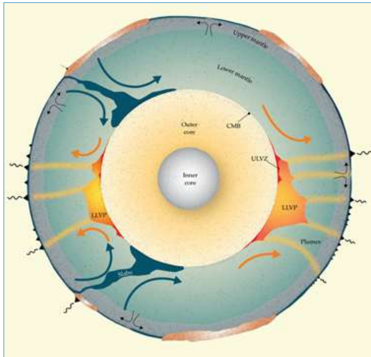
Fig. 1. The two continent-size formations extending about 1,200 km above the hot-core – mantel boundary
